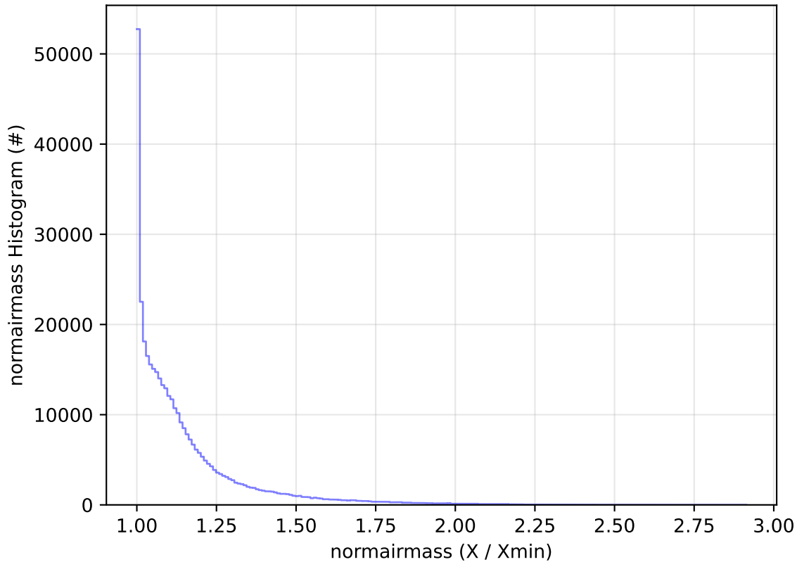
ddf_acor_sf25_lsf30_lsr10_v3.4_10yrs WFD y band: normairmass Histogram
