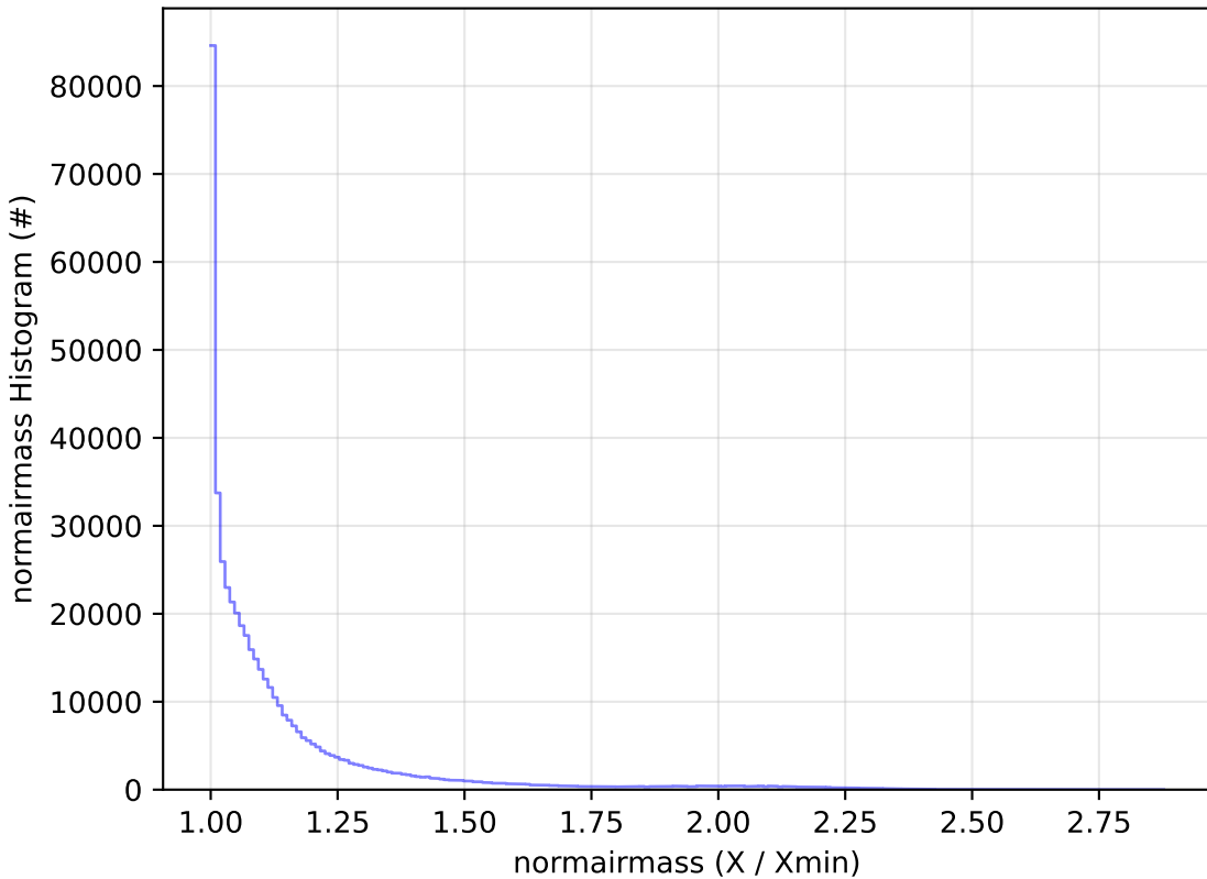
ddf_acor_sf25_lsf30_lsr10_v3.4_10yrs WFD r band: normairmass Histogram
