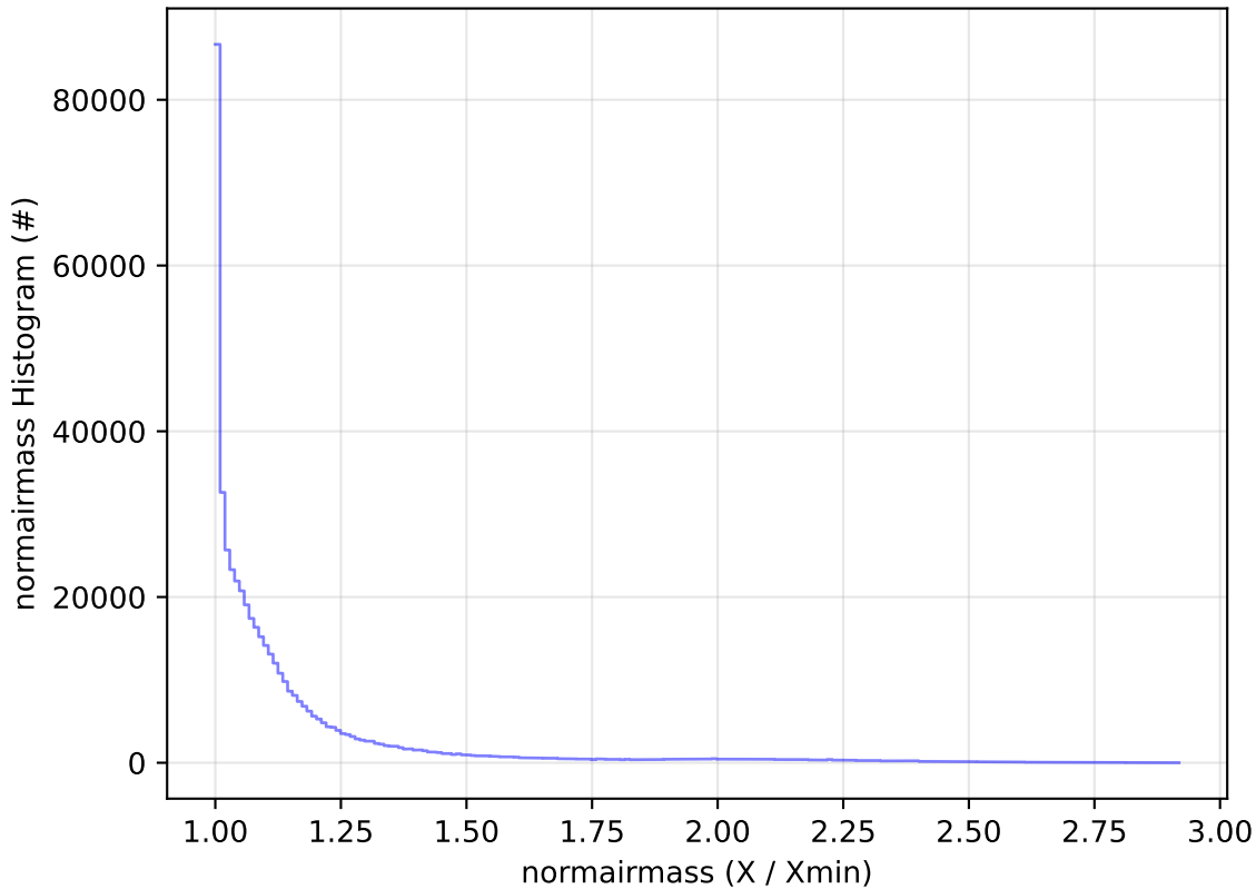
ddf_acor_sf25_lsf30_lsr10_v3.4_10yrs WFD i band: normairmass Histogram
