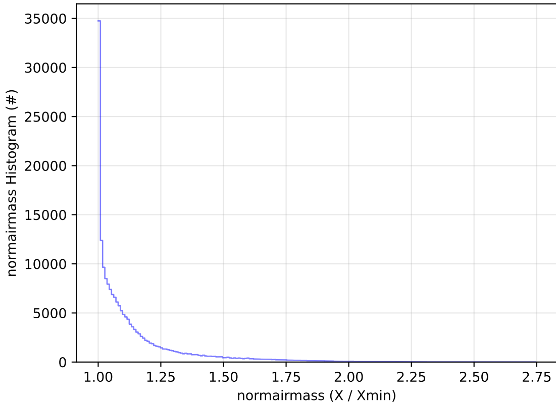
ddf_acor_sf25_lsf30_lsr10_v3.4_10yrs WFD g band: normairmass Histogram
