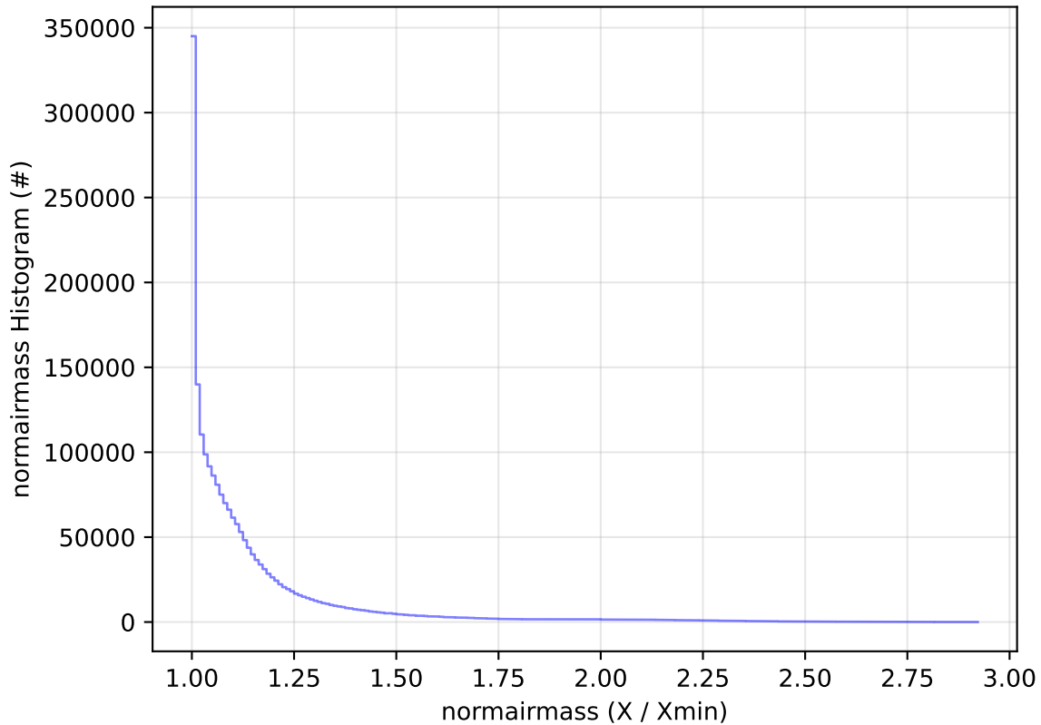
ddf_acor_sf25_lsf30_lsr10_v3.4_10yrs WFD all bands: normairmass Histogram
