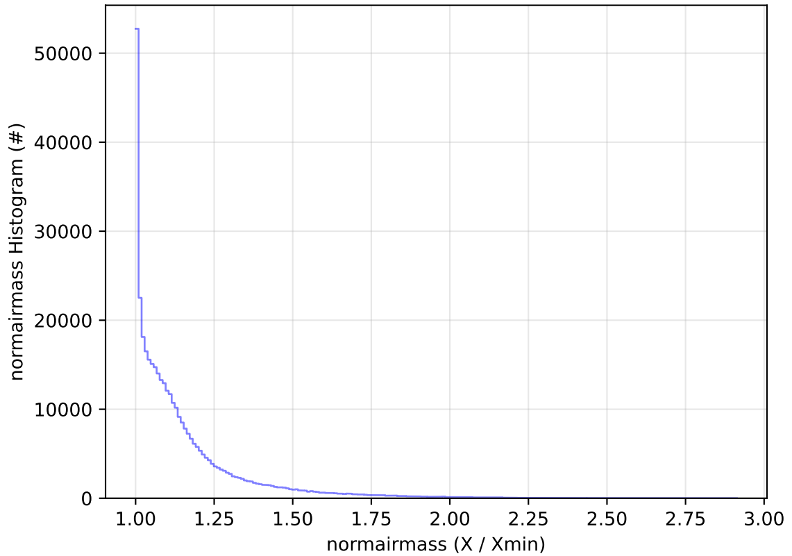
ddf_acor_sf25_lsf30_lsr10_v3.4_10yrs All sky y band: normairmass Histogram
