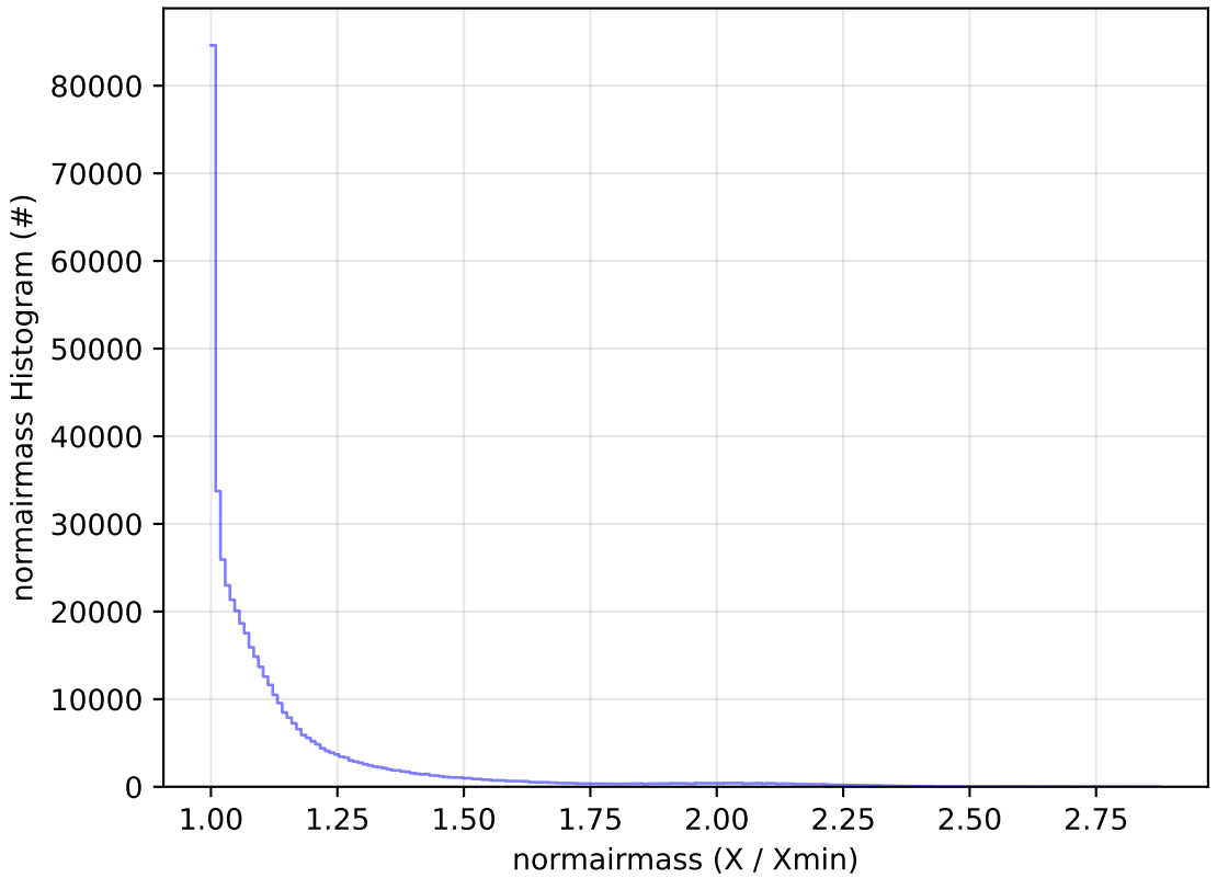
ddf_acor_sf25_lsf30_lsr10_v3.4_10yrs All sky r band: normairmass Histogram
