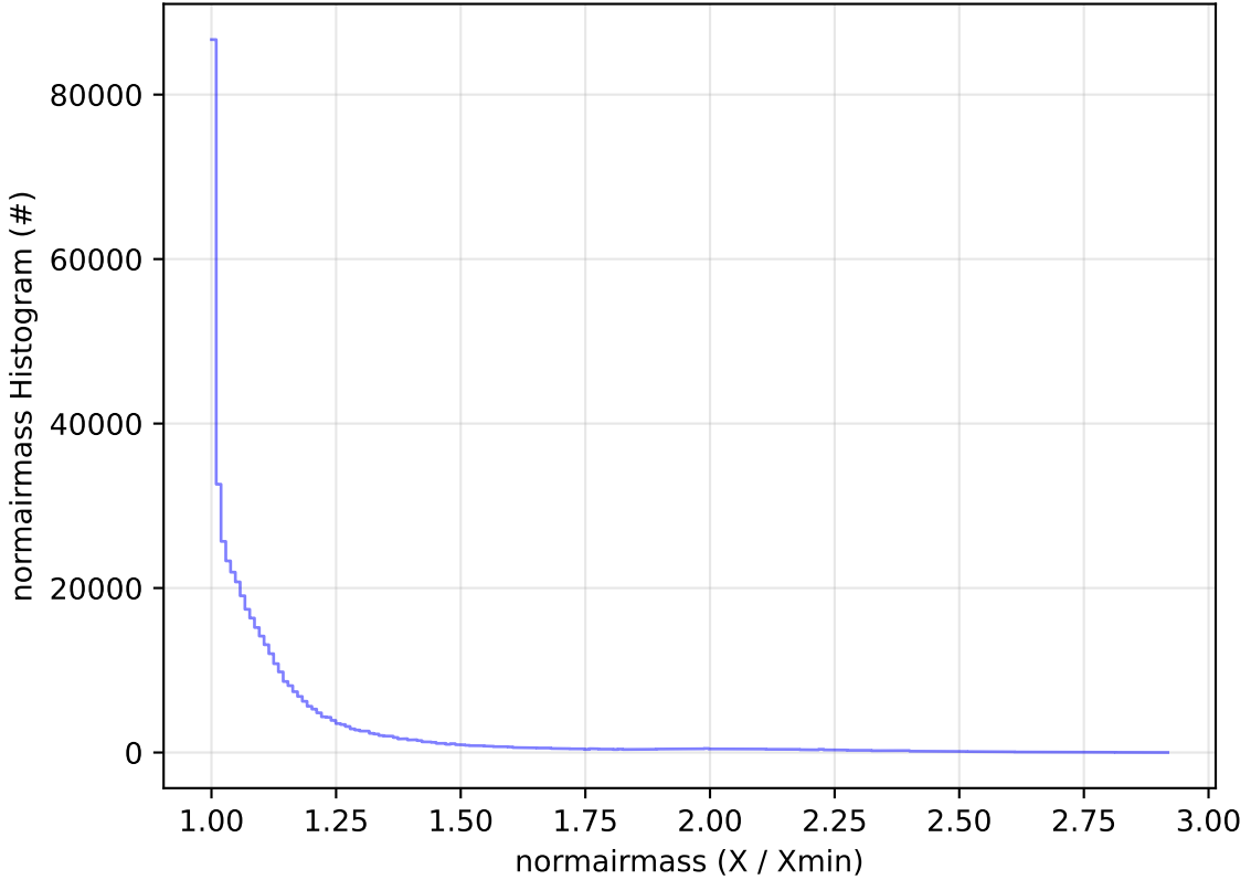
ddf_acor_sf25_lsf30_lsr10_v3.4_10yrs All sky i band: normairmass Histogram
