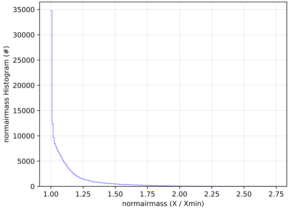
ddf_acor_sf25_lsf30_lsr10_v3.4_10yrs All sky g band: normairmass Histogram
