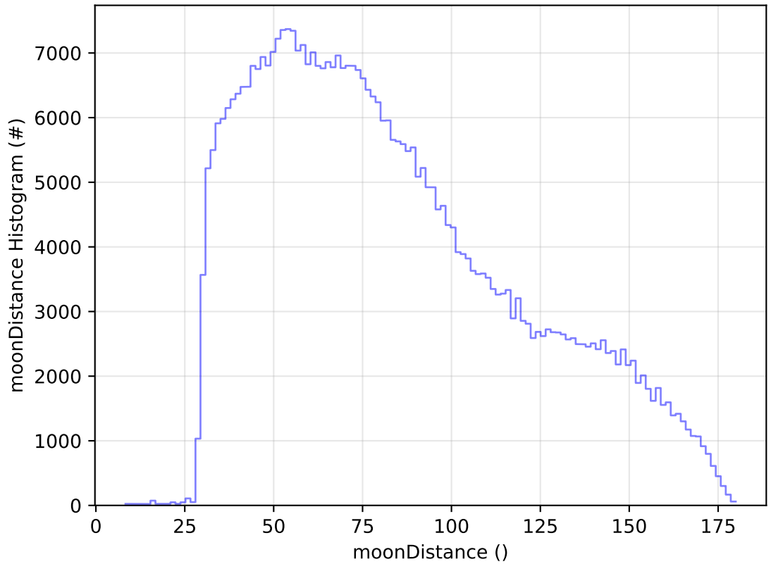
ddf_acor_sf25_lsf30_lsr10_v3.4_10yrs WFD z band: moonDistance Histogram
