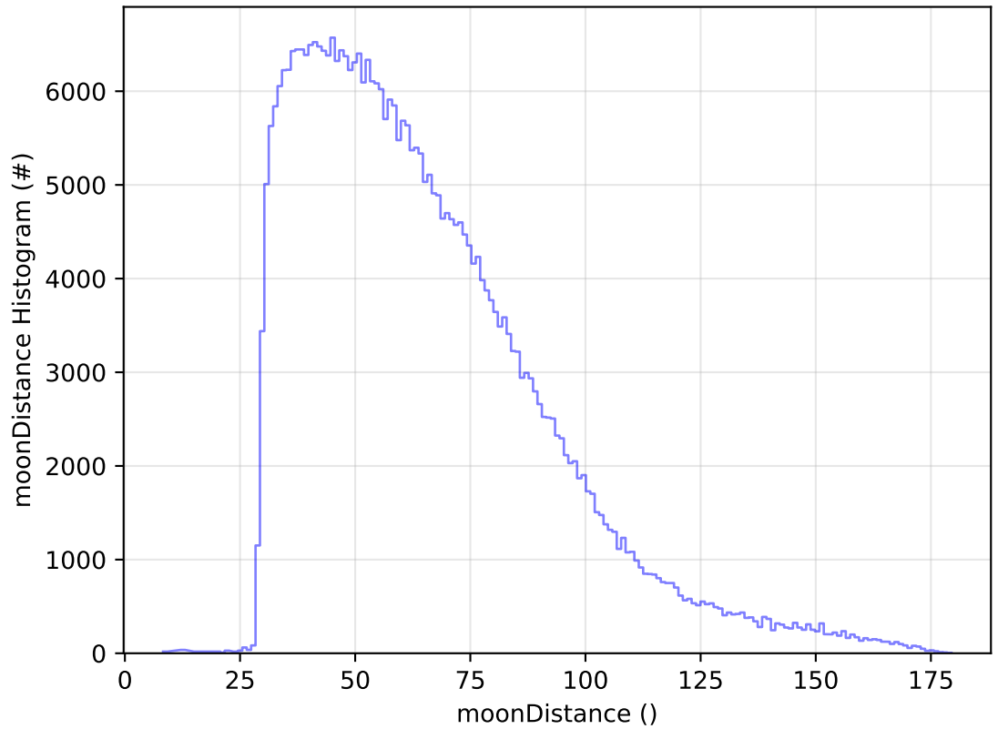
ddf_acor_sf25_lsf30_lsr10_v3.4_10yrs WFD y band: moonDistance Histogram
