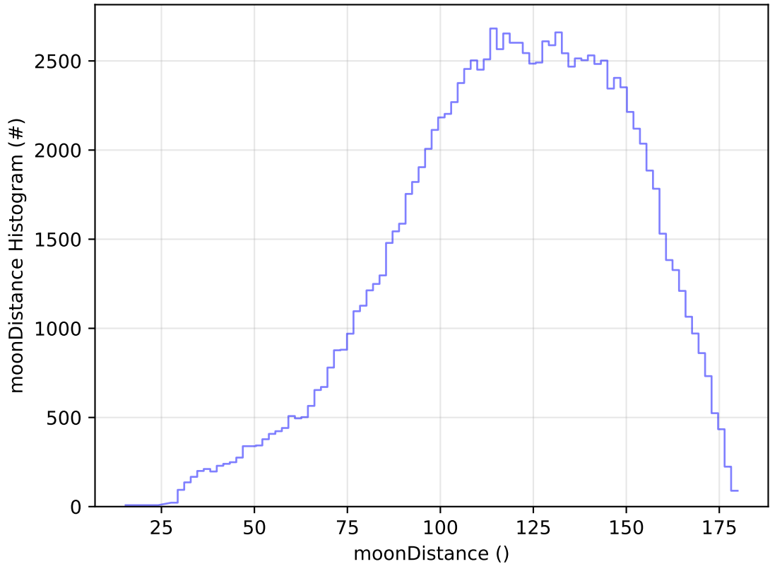
ddf_acor_sf25_lsf30_lsr10_v3.4_10yrs WFD u band: moonDistance Histogram
