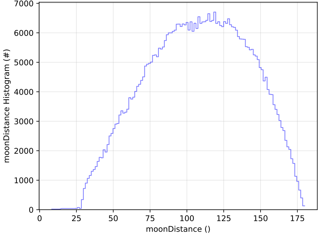
ddf_acor_sf25_lsf30_lsr10_v3.4_10yrs WFD r band: moonDistance Histogram
