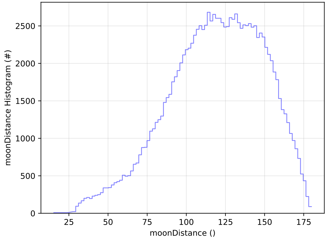
ddf_acor_sf25_lsf30_lsr10_v3.4_10yrs All sky u band: moonDistance Histogram
