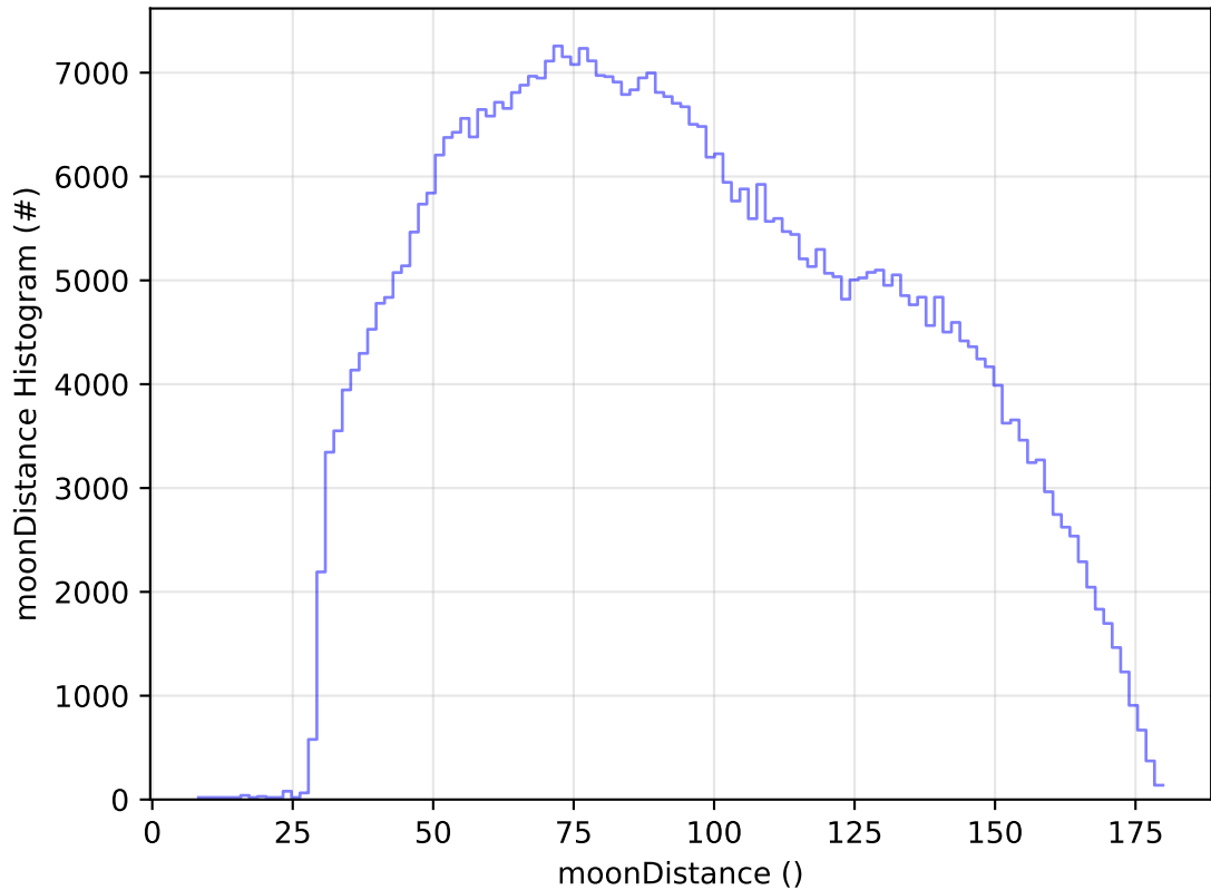
ddf_acor_sf25_lsf30_lsr10_v3.4_10yrs All sky i band: moonDistance Histogram
