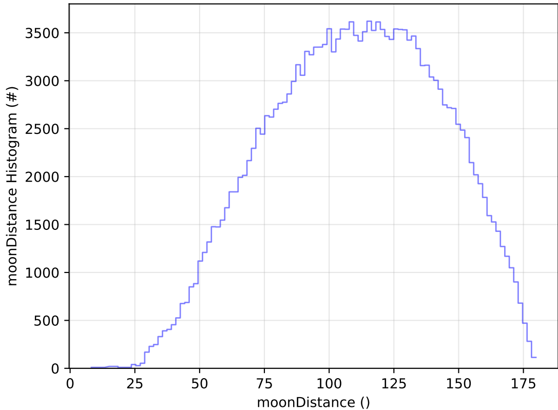
ddf_acor_sf25_lsf30_lsr10_v3.4_10yrs All sky g band: moonDistance Histogram
