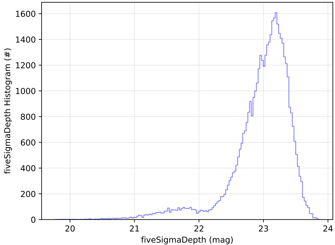
ddf_acor_sf25_lsf30_lsr10_v3.4_10yrs Yr 1 z band: fiveSigmaDepth Histogram
