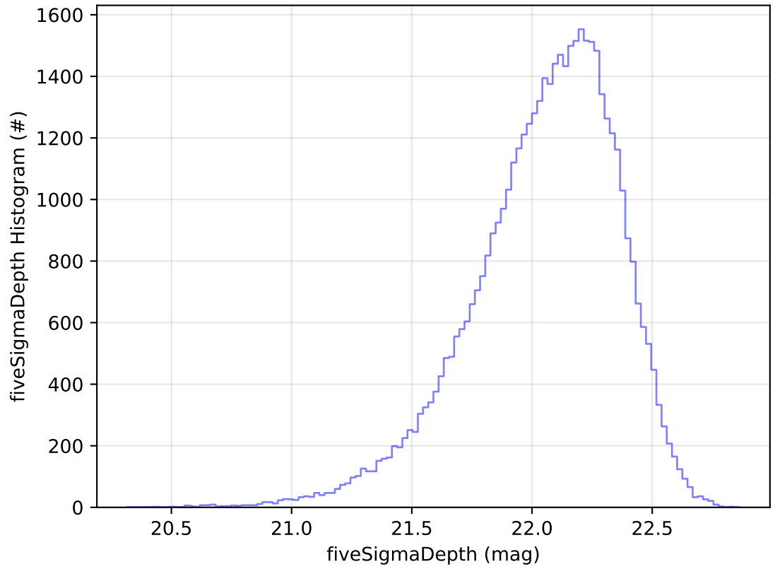
ddf_acor_sf25_lsf30_lsr10_v3.4_10yrs Yr 1 y band: fiveSigmaDepth Histogram
