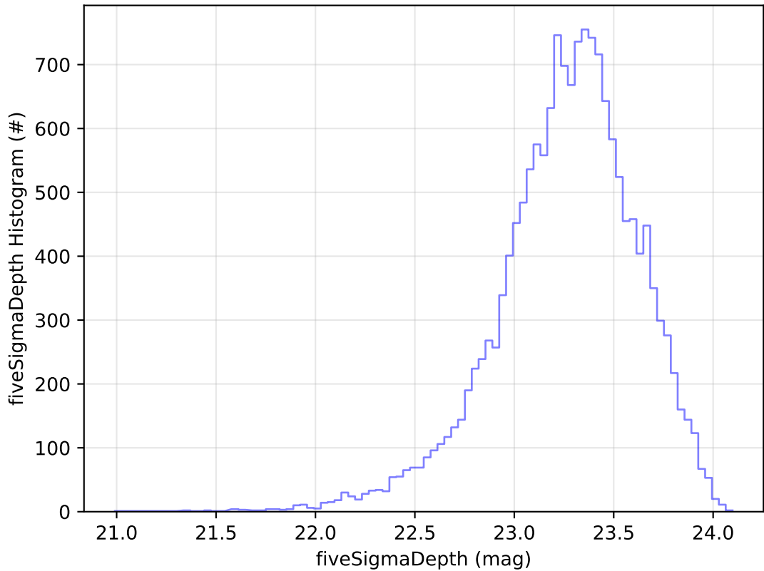
ddf_acor_sf25_lsf30_lsr10_v3.4_10yrs Yr 1 u band: fiveSigmaDepth Histogram
