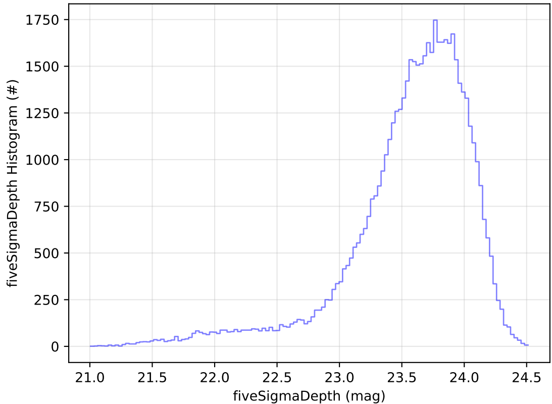
ddf_acor_sf25_lsf30_lsr10_v3.4_10yrs Yr 1 i band: fiveSigmaDepth Histogram
