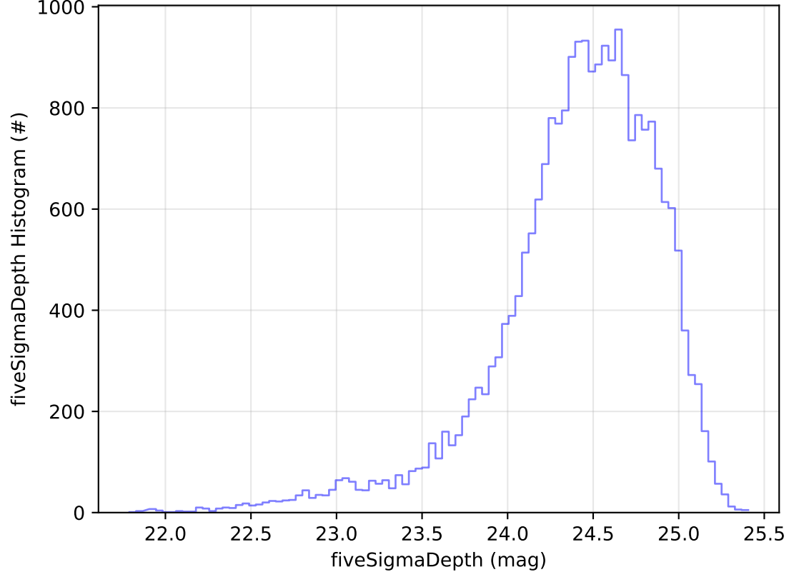
ddf_acor_sf25_lsf30_lsr10_v3.4_10yrs Yr 1 g band: fiveSigmaDepth Histogram
