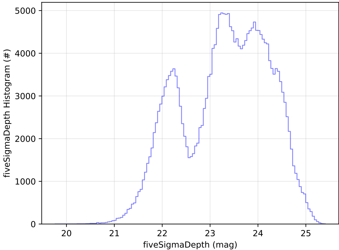
ddf_acor_sf25_lsf30_lsr10_v3.4_10yrs Yr 1 all bands: fiveSigmaDepth Histogram
