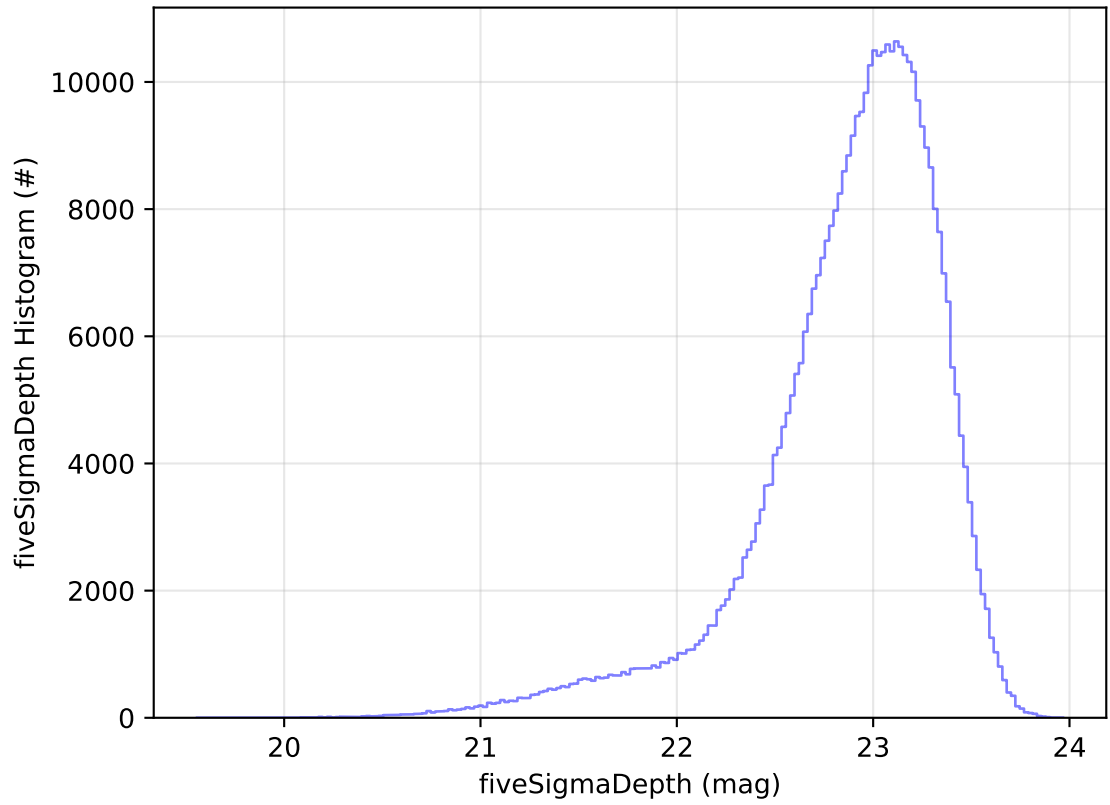
ddf_acor_sf25_lsf30_lsr10_v3.4_10yrs WFD z band: fiveSigmaDepth Histogram
