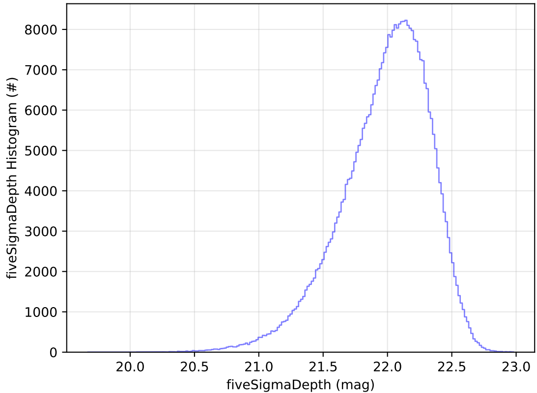
ddf_acor_sf25_lsf30_lsr10_v3.4_10yrs WFD y band: fiveSigmaDepth Histogram
