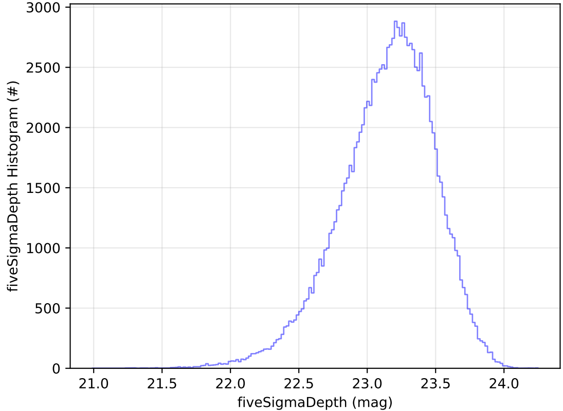
ddf_acor_sf25_lsf30_lsr10_v3.4_10yrs WFD u band: fiveSigmaDepth Histogram
