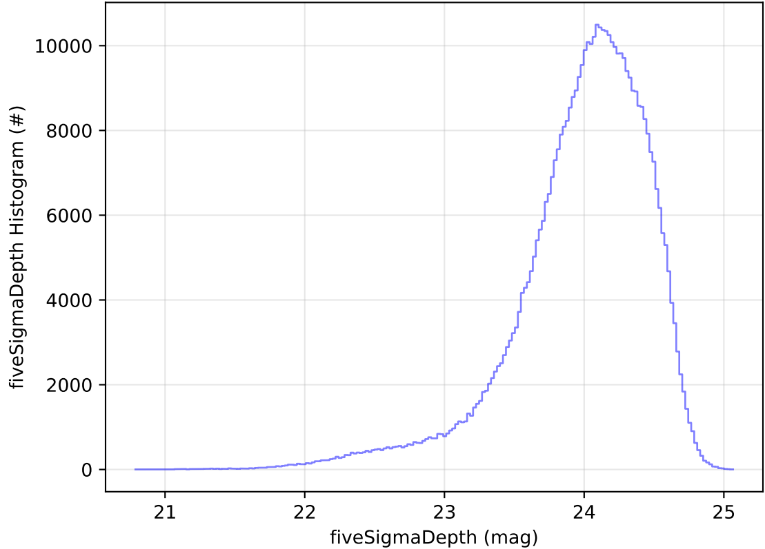
ddf_acor_sf25_lsf30_lsr10_v3.4_10yrs WFD r band: fiveSigmaDepth Histogram
