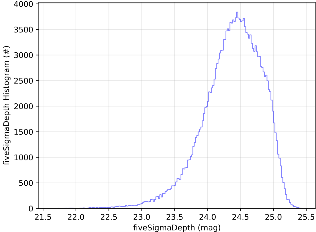
ddf_acor_sf25_lsf30_lsr10_v3.4_10yrs WFD g band: fiveSigmaDepth Histogram
