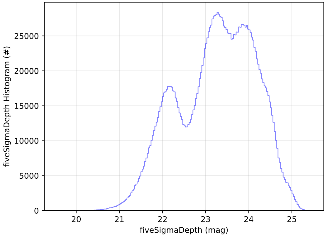
ddf_acor_sf25_lsf30_lsr10_v3.4_10yrs WFD all bands: fiveSigmaDepth Histogram
