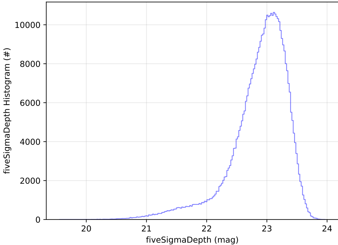
ddf_acor_sf25_lsf30_lsr10_v3.4_10yrs All sky z band: fiveSigmaDepth Histogram
