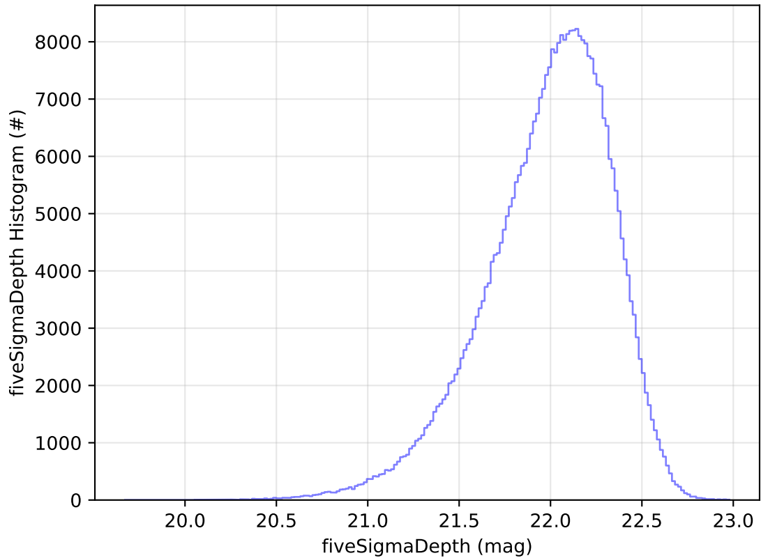
ddf_acor_sf25_lsf30_lsr10_v3.4_10yrs All sky y band: fiveSigmaDepth Histogram
