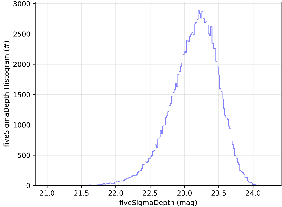
ddf_acor_sf25_lsf30_lsr10_v3.4_10yrs All sky u band: fiveSigmaDepth Histogram
