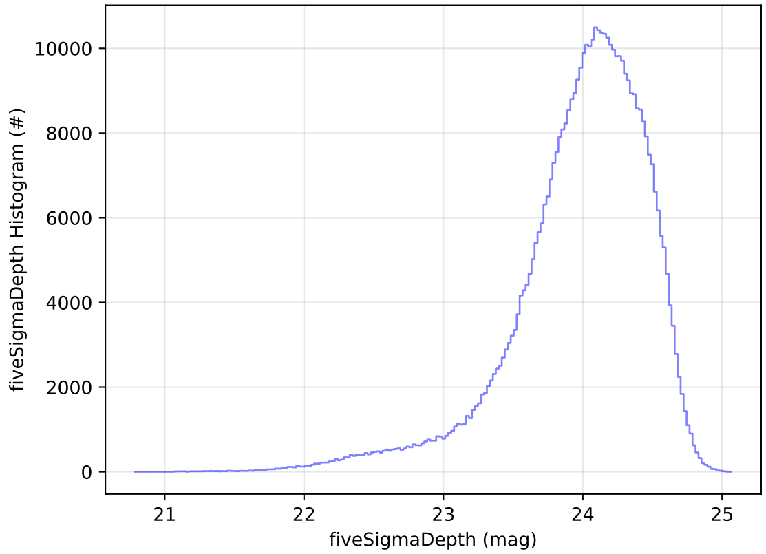
ddf_acor_sf25_lsf30_lsr10_v3.4_10yrs All sky r band: fiveSigmaDepth Histogram
