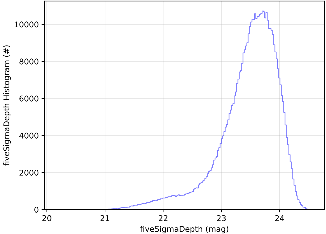
ddf_acor_sf25_lsf30_lsr10_v3.4_10yrs All sky i band: fiveSigmaDepth Histogram
