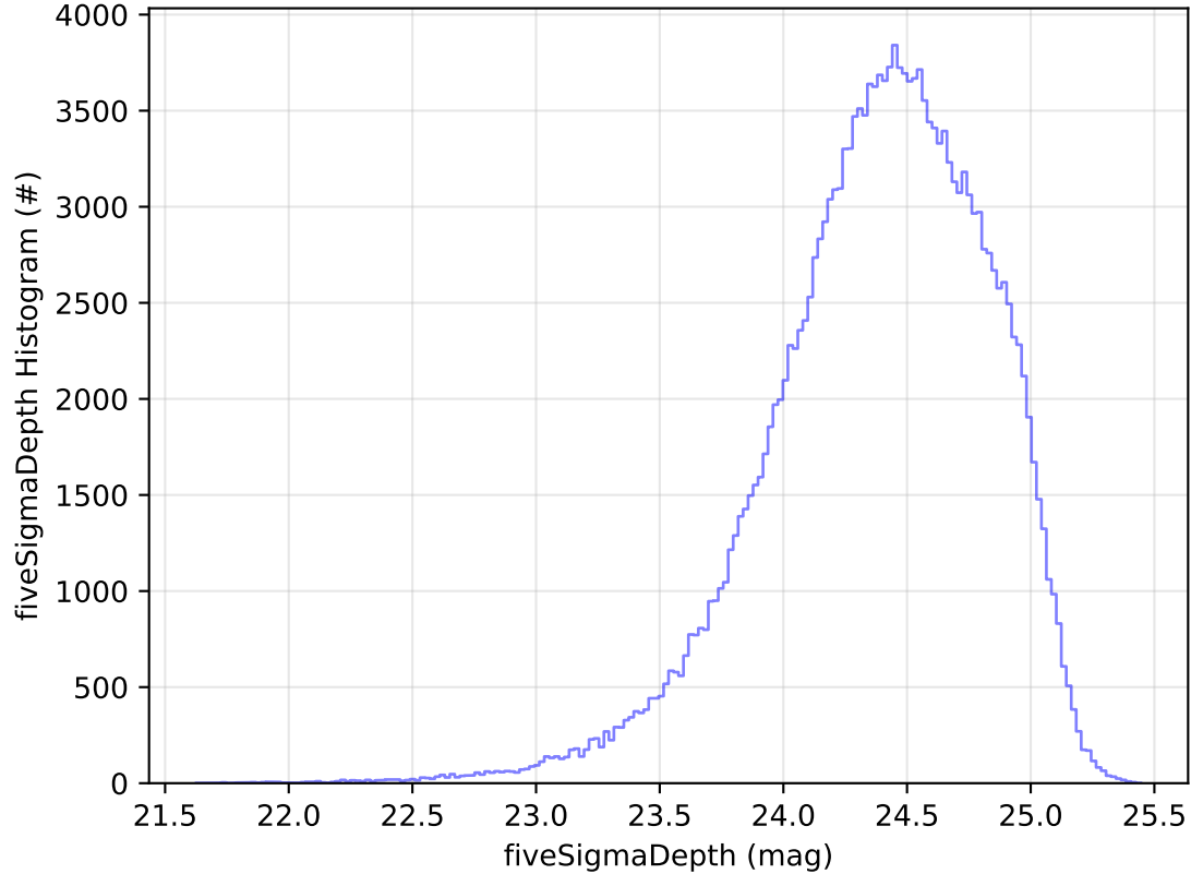
ddf_acor_sf25_lsf30_lsr10_v3.4_10yrs All sky g band: fiveSigmaDepth Histogram
