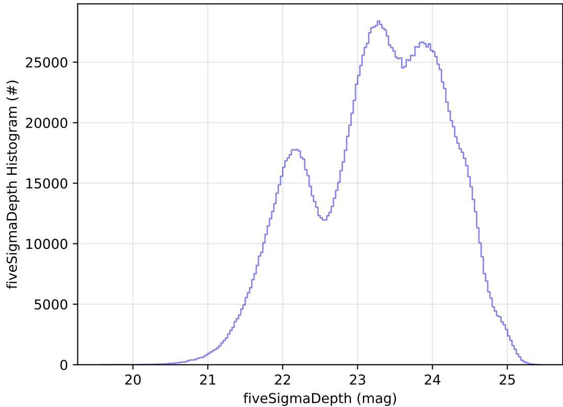
ddf_acor_sf25_lsf30_lsr10_v3.4_10yrs All sky all bands: fiveSigmaDepth Histogram
