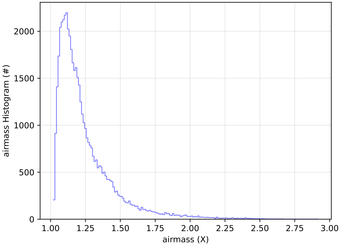
ddf_acor_sf25_lsf30_lsr10_v3.4_10yrs Yr 1 y band: airmass Histogram
