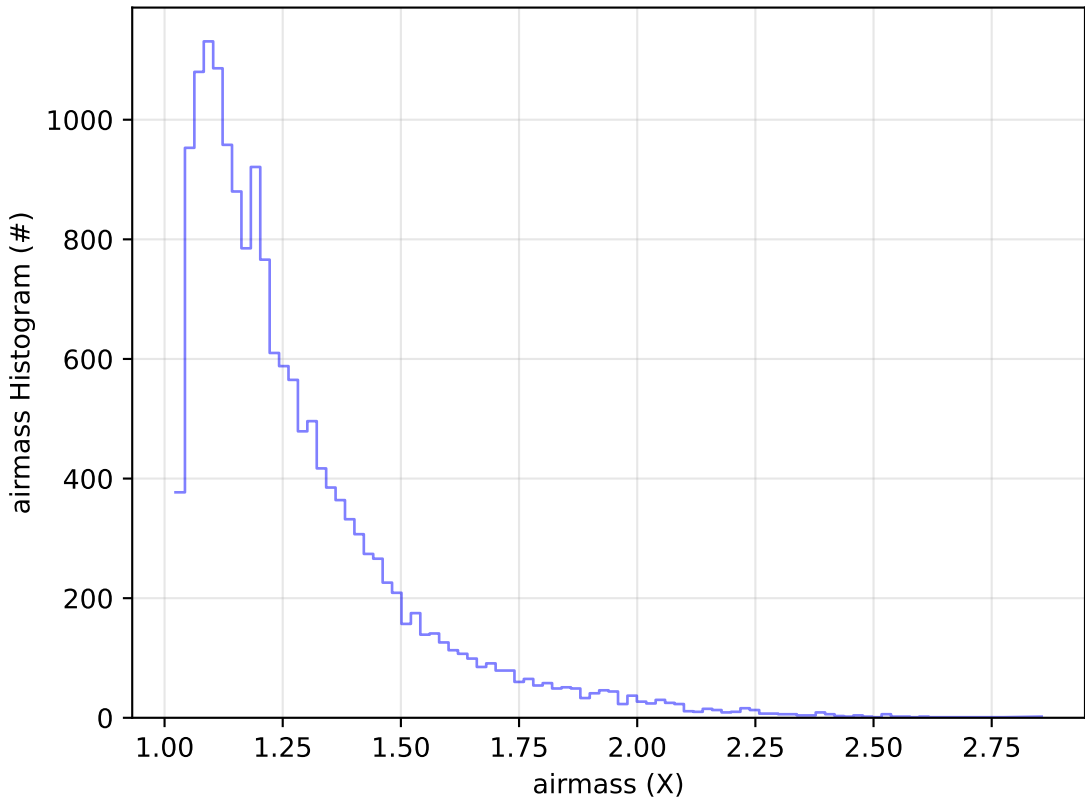
ddf_acor_sf25_lsf30_lsr10_v3.4_10yrs Yr 1 u band: airmass Histogram
