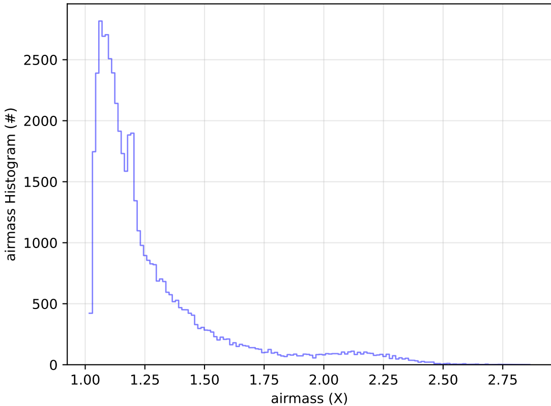
ddf_acor_sf25_lsf30_lsr10_v3.4_10yrs Yr 1 r band: airmass Histogram
