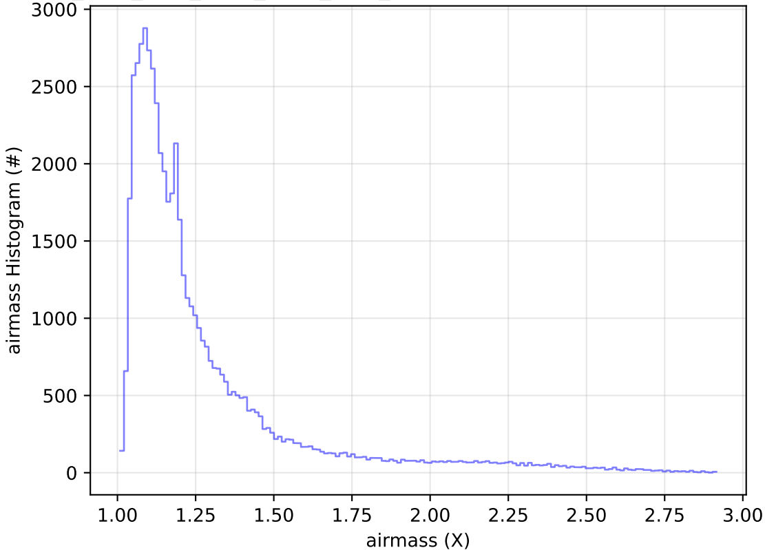
ddf_acor_sf25_lsf30_lsr10_v3.4_10yrs Yr 1 i band: airmass Histogram
