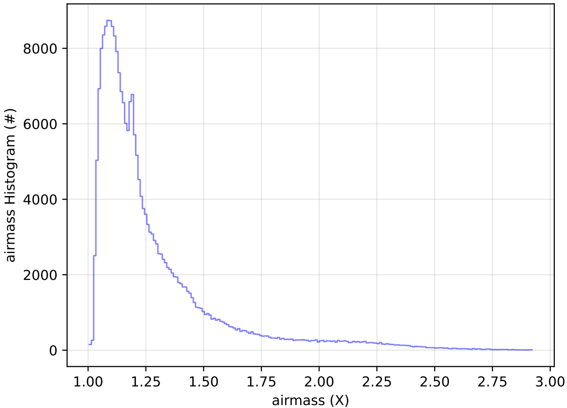
ddf_acor_sf25_lsf30_lsr10_v3.4_10yrs Yr 1 all bands: airmass Histogram
