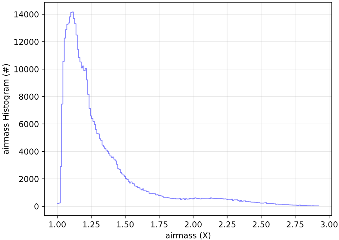
ddf_acor_sf25_lsf30_lsr10_v3.4_10yrs WFD z band: airmass Histogram
