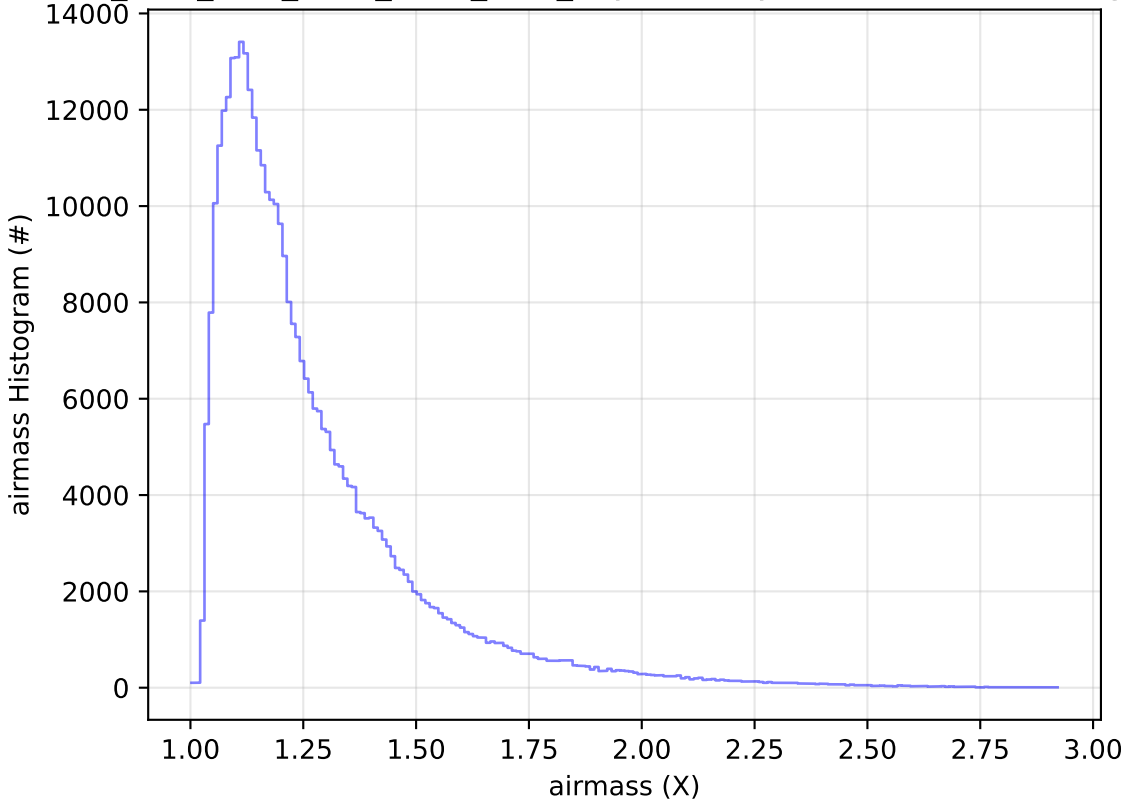
ddf_acor_sf25_lsf30_lsr10_v3.4_10yrs WFD y band: airmass Histogram
