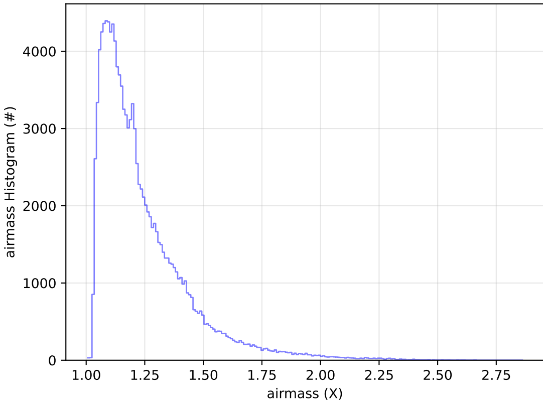
ddf_acor_sf25_lsf30_lsr10_v3.4_10yrs WFD u band: airmass Histogram
