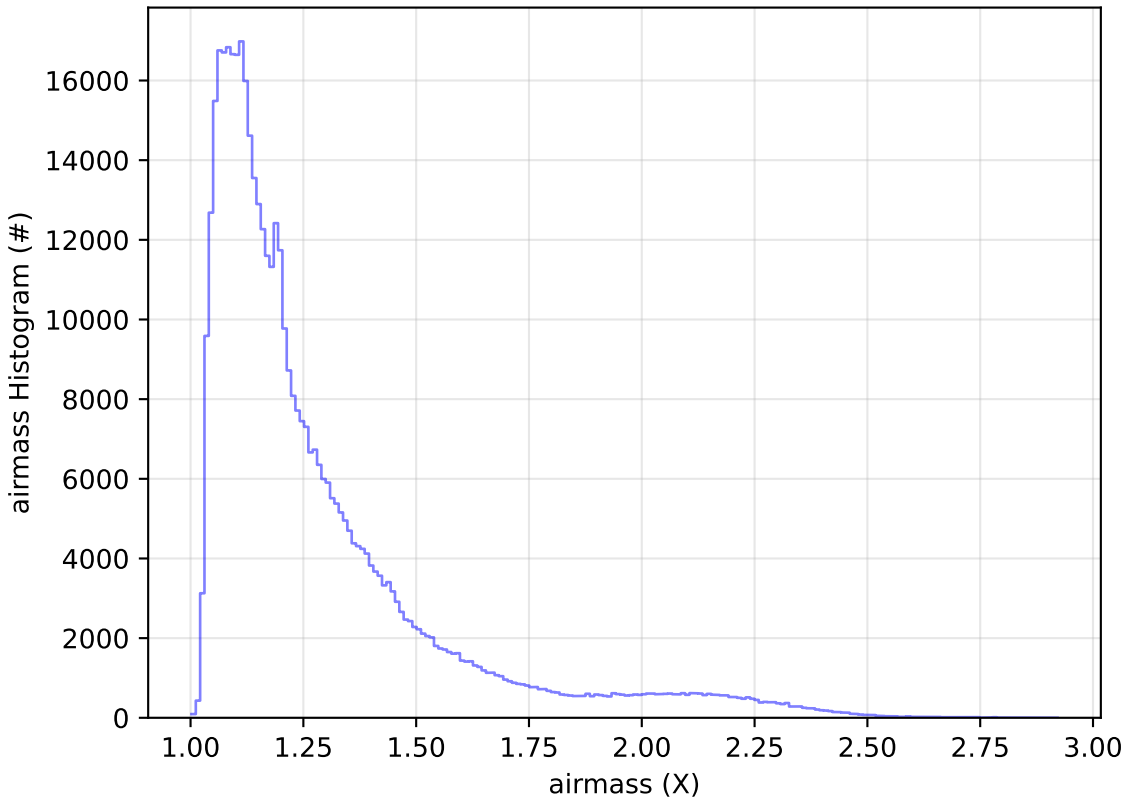
ddf_acor_sf25_lsf30_lsr10_v3.4_10yrs WFD r band: airmass Histogram
