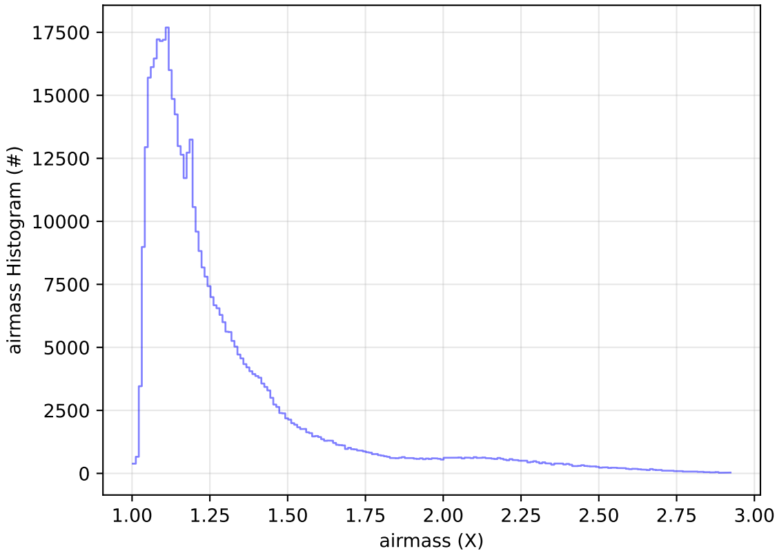
ddf_acor_sf25_lsf30_lsr10_v3.4_10yrs WFD i band: airmass Histogram
