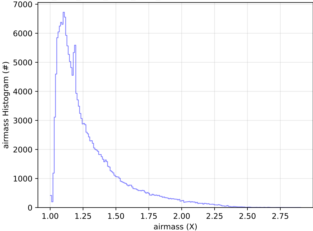
ddf_acor_sf25_lsf30_lsr10_v3.4_10yrs WFD g band: airmass Histogram
