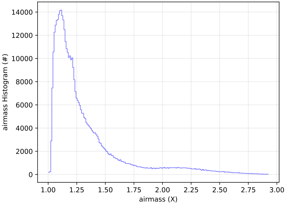
ddf_acor_sf25_lsf30_lsr10_v3.4_10yrs All sky z band: airmass Histogram
