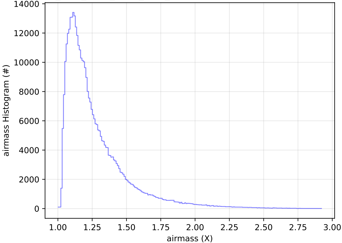
ddf_acor_sf25_lsf30_lsr10_v3.4_10yrs All sky y band: airmass Histogram
