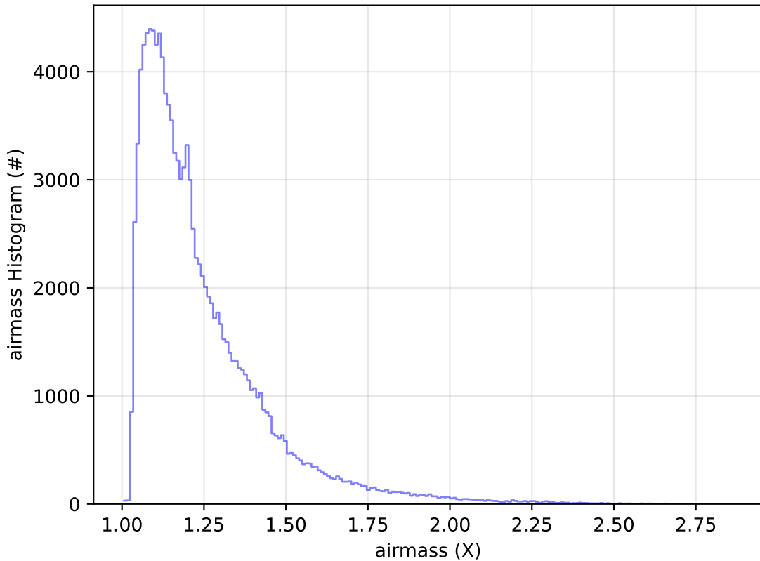
ddf_acor_sf25_lsf30_lsr10_v3.4_10yrs All sky u band: airmass Histogram
