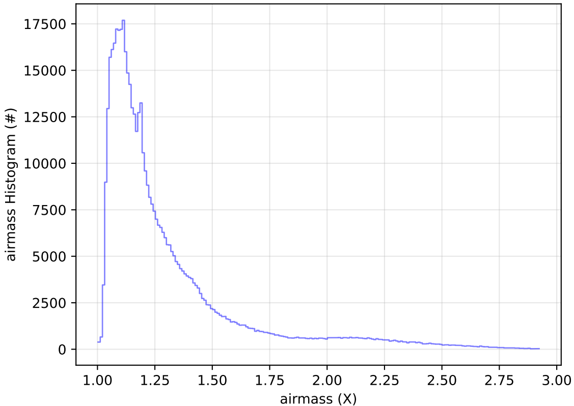
ddf_acor_sf25_lsf30_lsr10_v3.4_10yrs All sky i band: airmass Histogram
